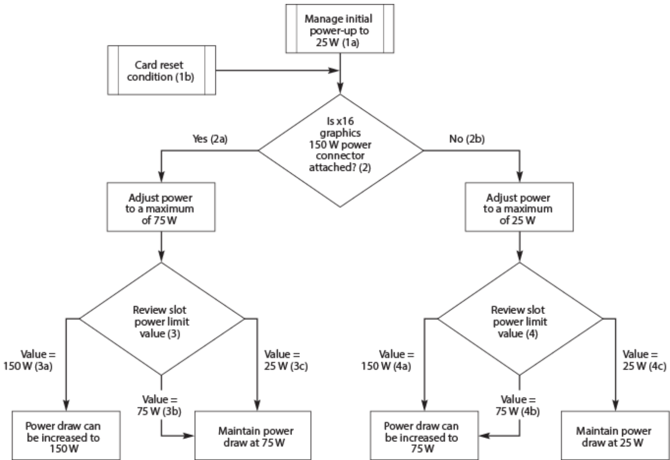
Figure 32: PCI Express 150 W Add-in Card Power-Up Sequence
