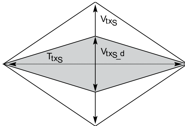
1308 Figure 26: 5.0 GT/s System Board Transmitter Path Composite Compliance Eye Diagram
