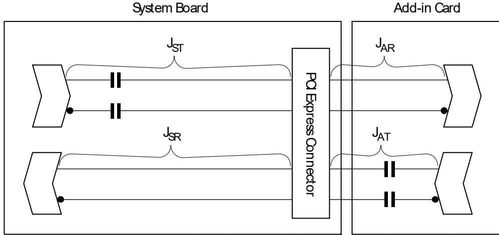
Figure 19: Jitter Budget
