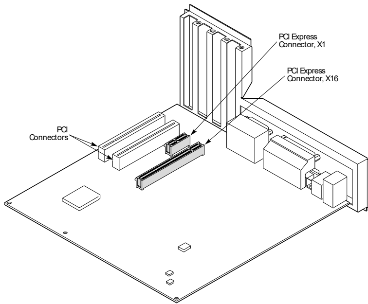
Figure 85: More PCI Express Connectors are Introduced on a microATX System Board
