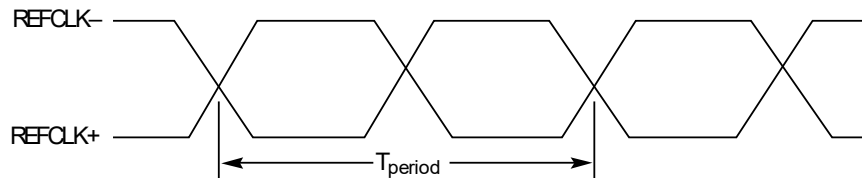
Figure 5: Differential REFCLK Waveform
