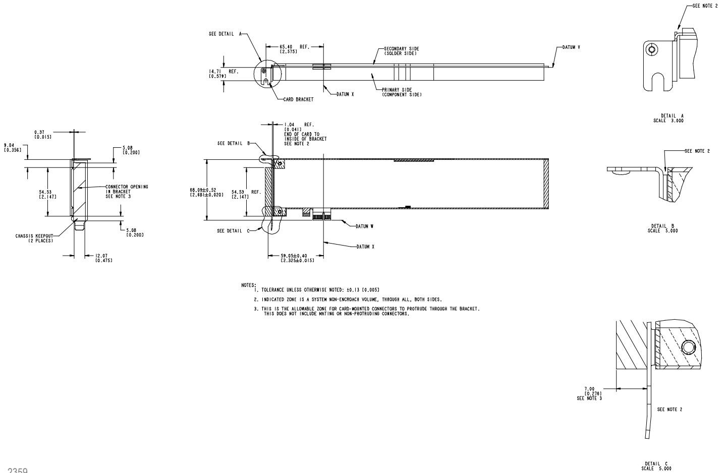
Figure 68: Low Profile PCI Express Add-in Card with the I/O Bracket
