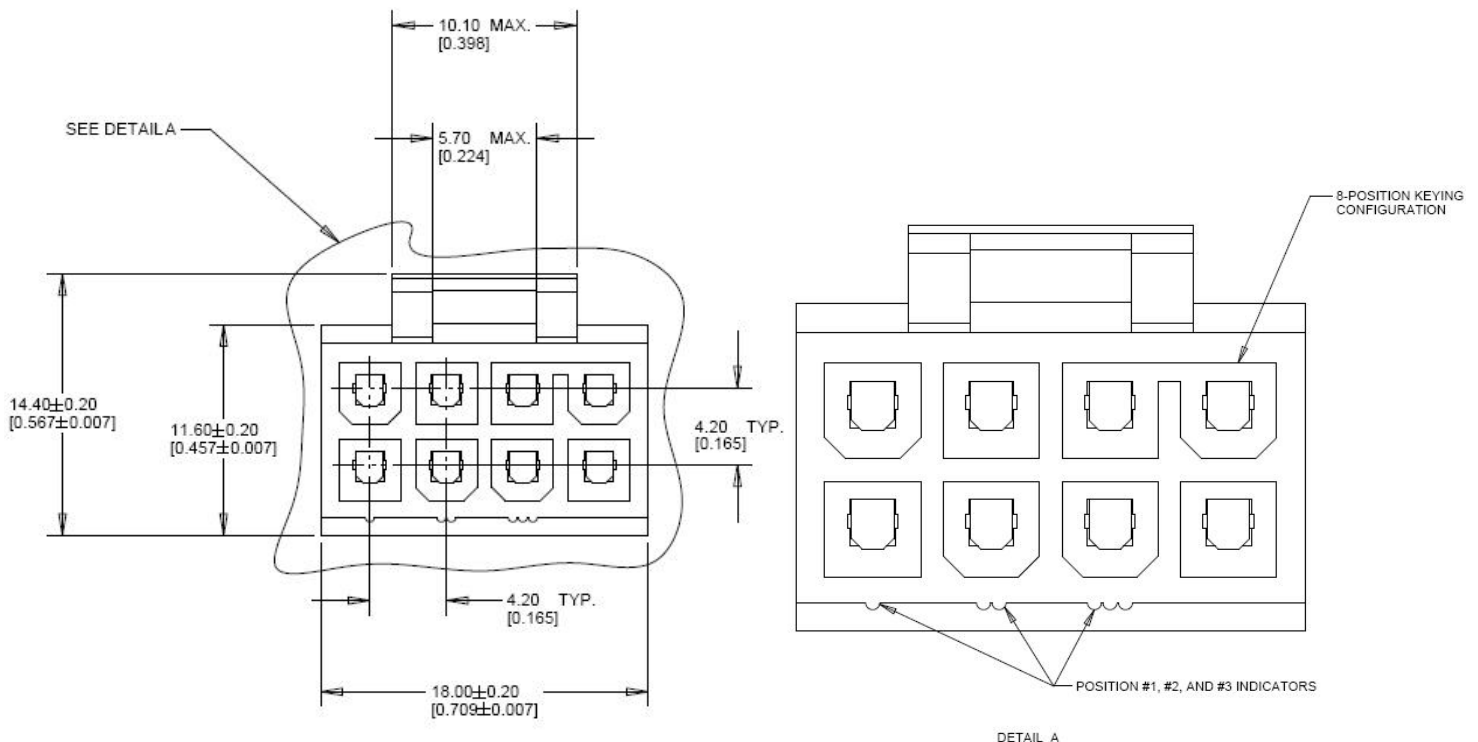
Figure 56: Modular Plug Connector Housing (All Dimensions in mm [Inches])
