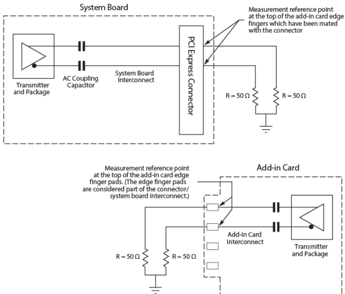
Figure 101 Example Interconnect Terminated at the Connector Interface
