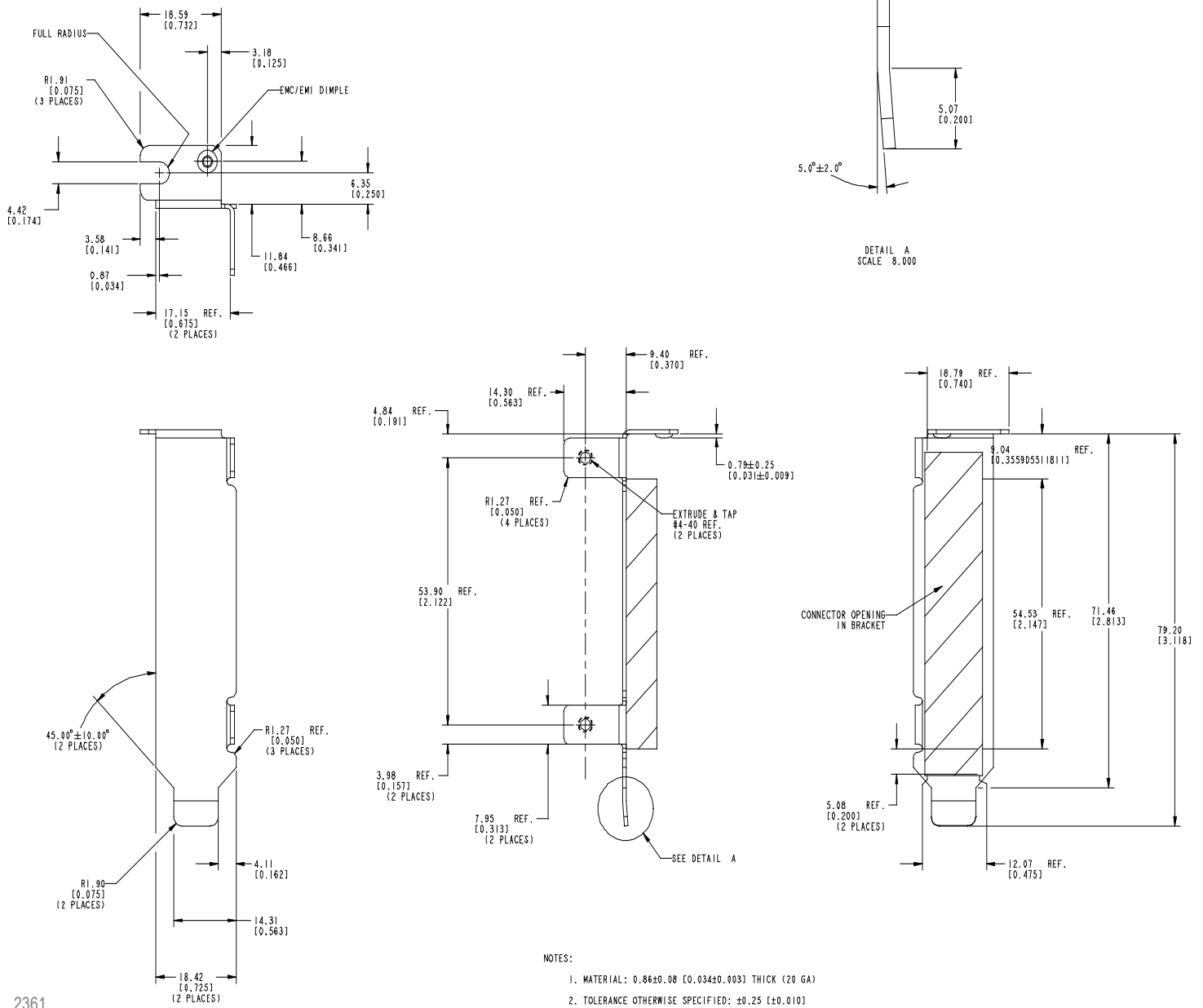
Figure 69: Low Profile I/O Bracket
