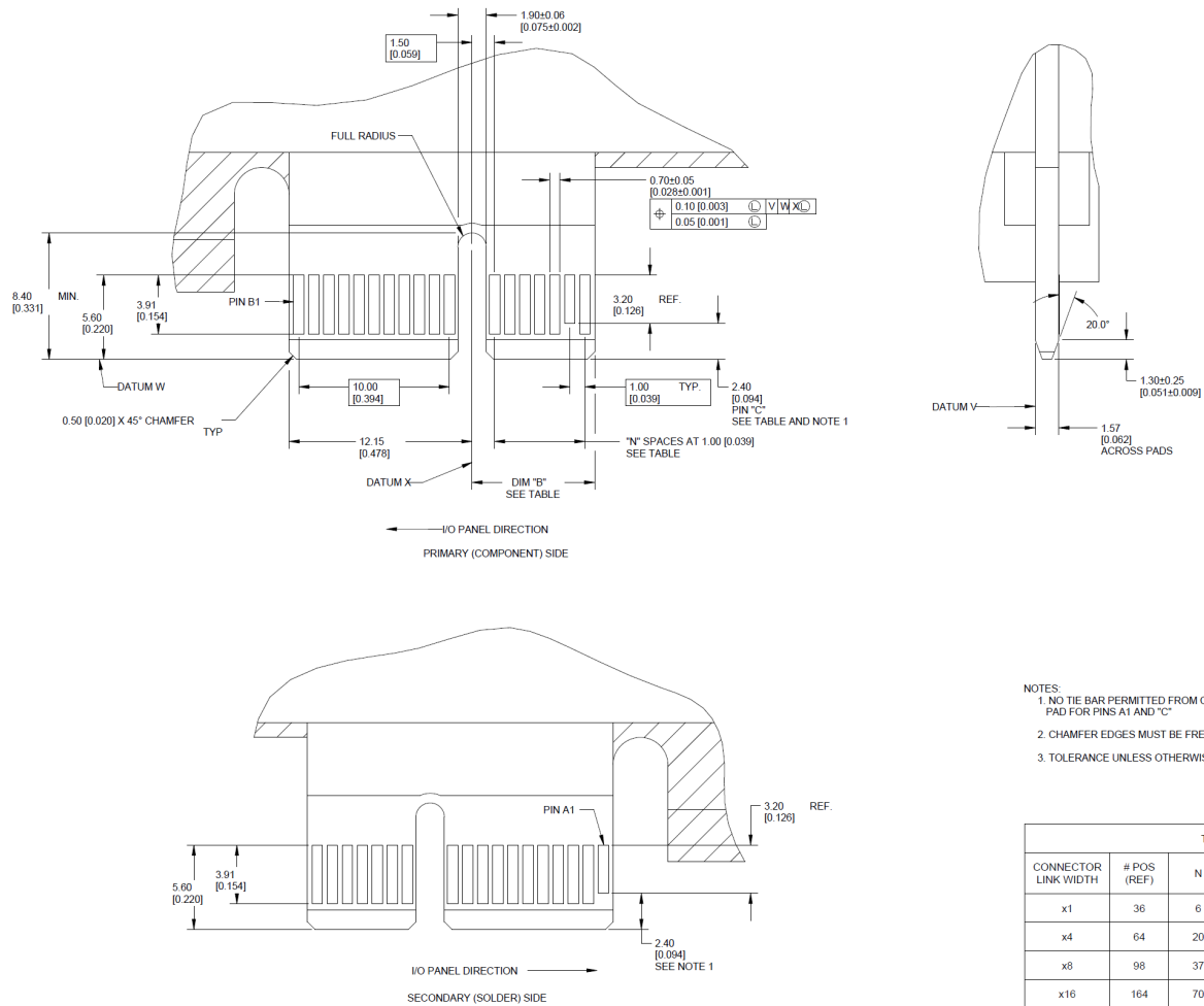
Figure 37: Add-in Card Edge-Finger Dimensions
