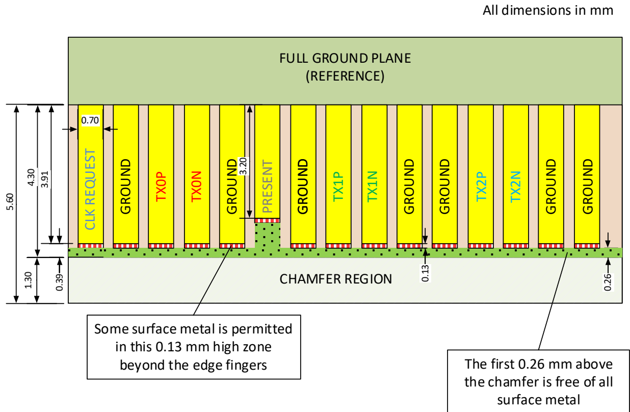
Figure 78: Add-in Card Edge-fingers Indicating Edge-finger Length and Surface Metal Keepout Areas
