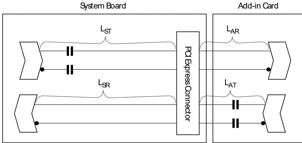
Figure 102. Insertion Loss Budgets
