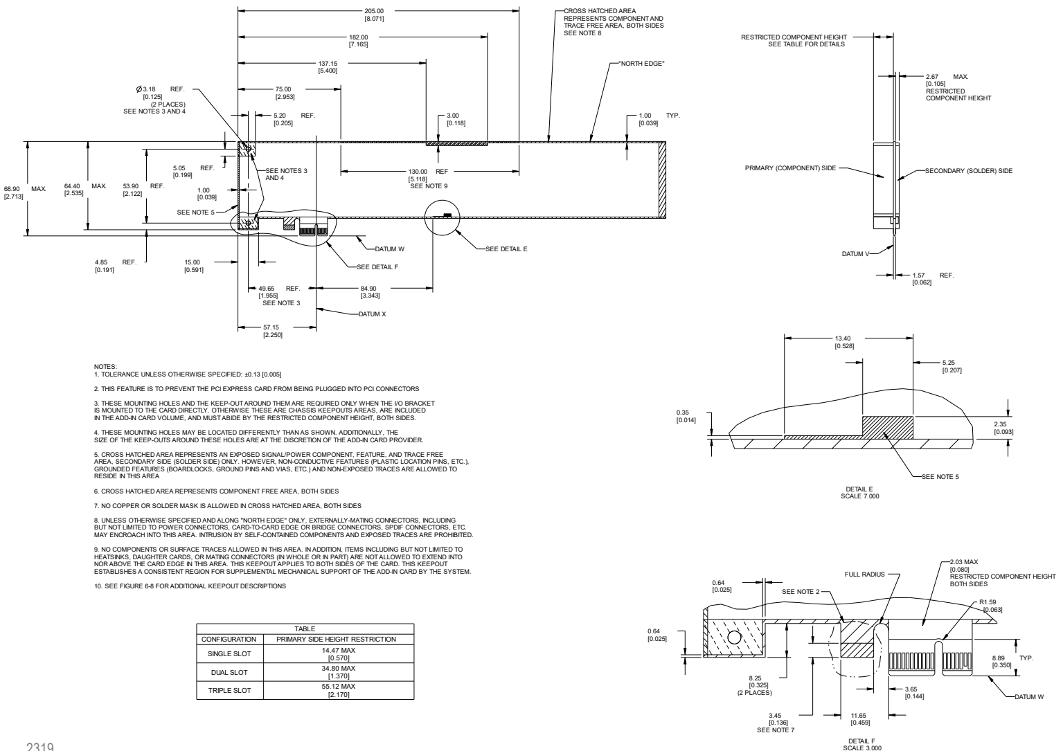
Figure 61: Standard Height PCI Express Add-in Card without the I/O Bracket
