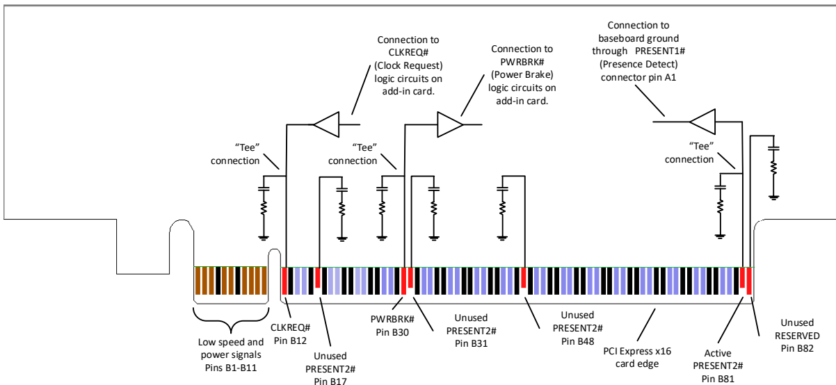
Figure 81: Add-in Card with AC Terminations on All Auxiliary and Reserved Signal Conductors. Only the B-side is shown.
